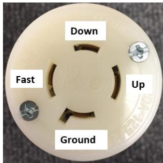
Plug Schematic
