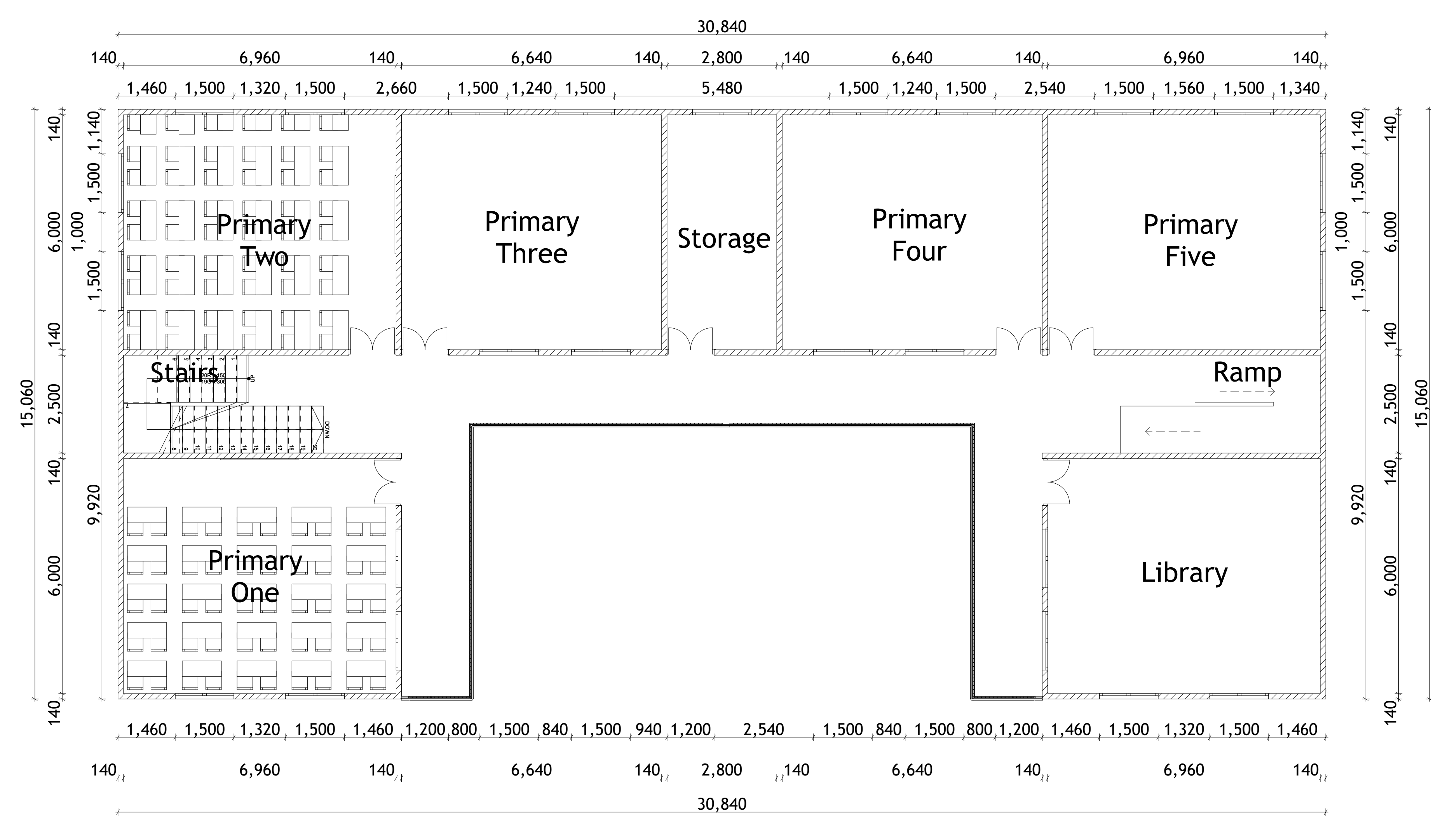
Classroom Block (First Floor) On Scale
