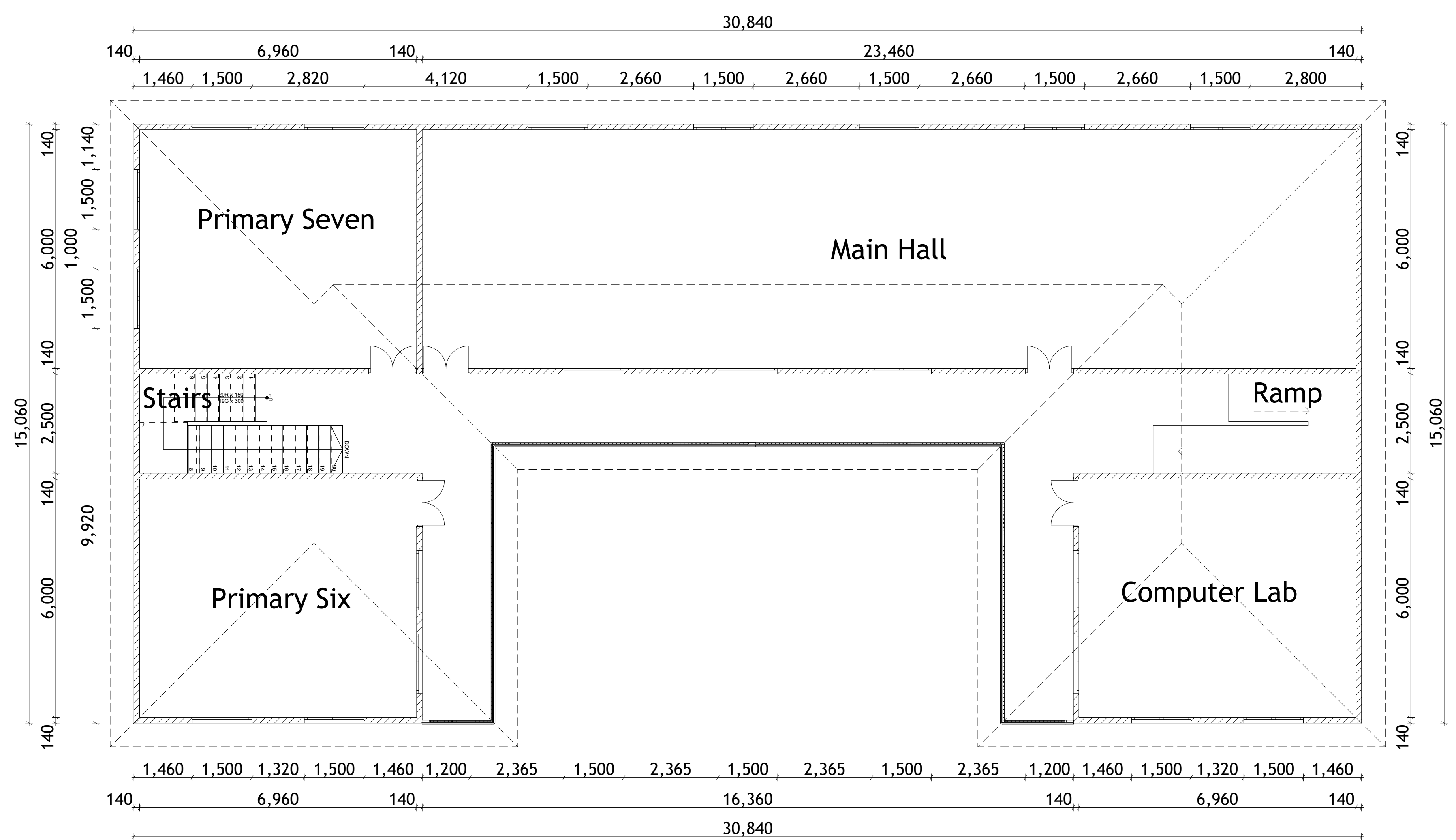
Classroom Block (Second Floor) On Scale
