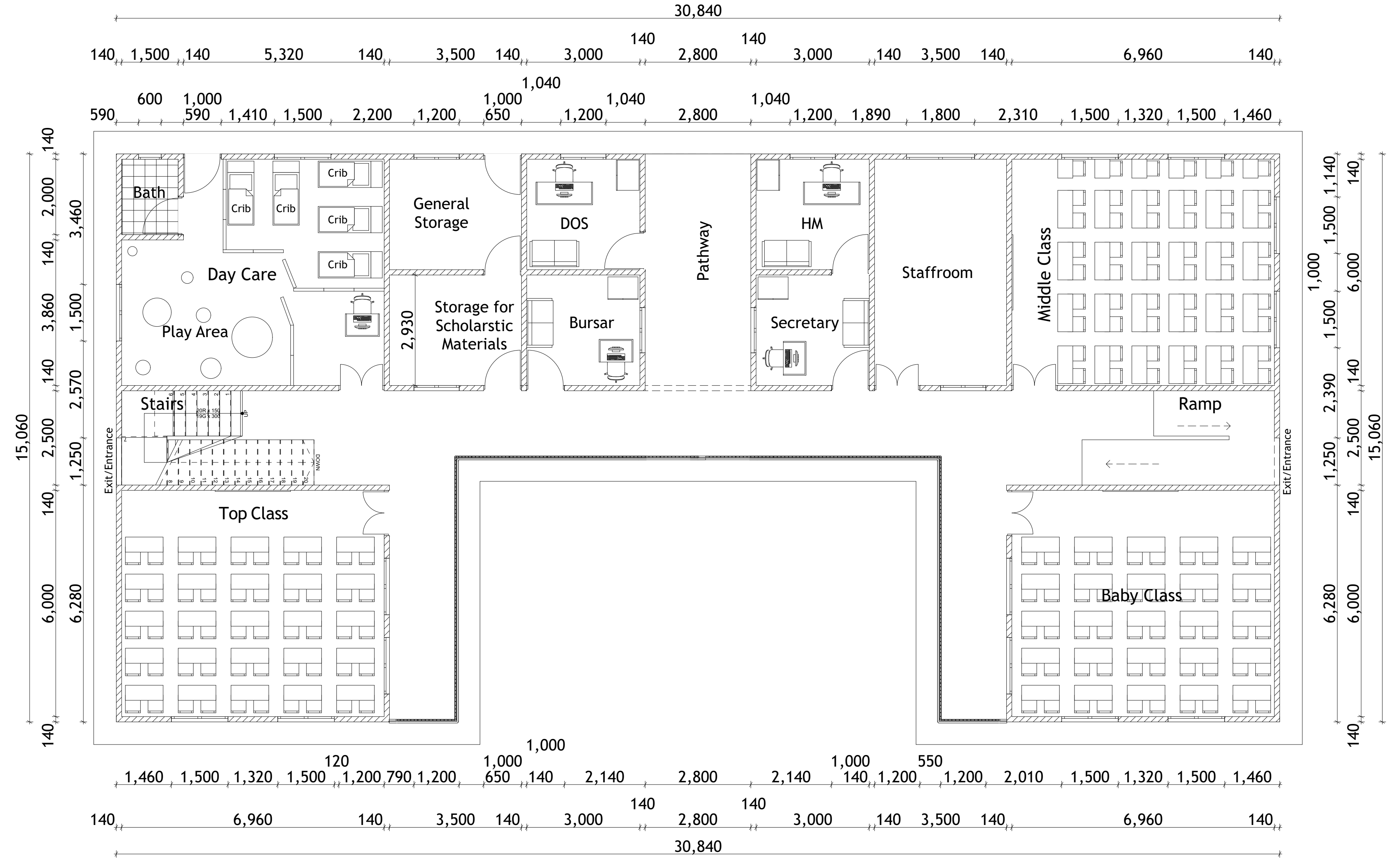
Classroom Block (Ground Floor) On Scale
