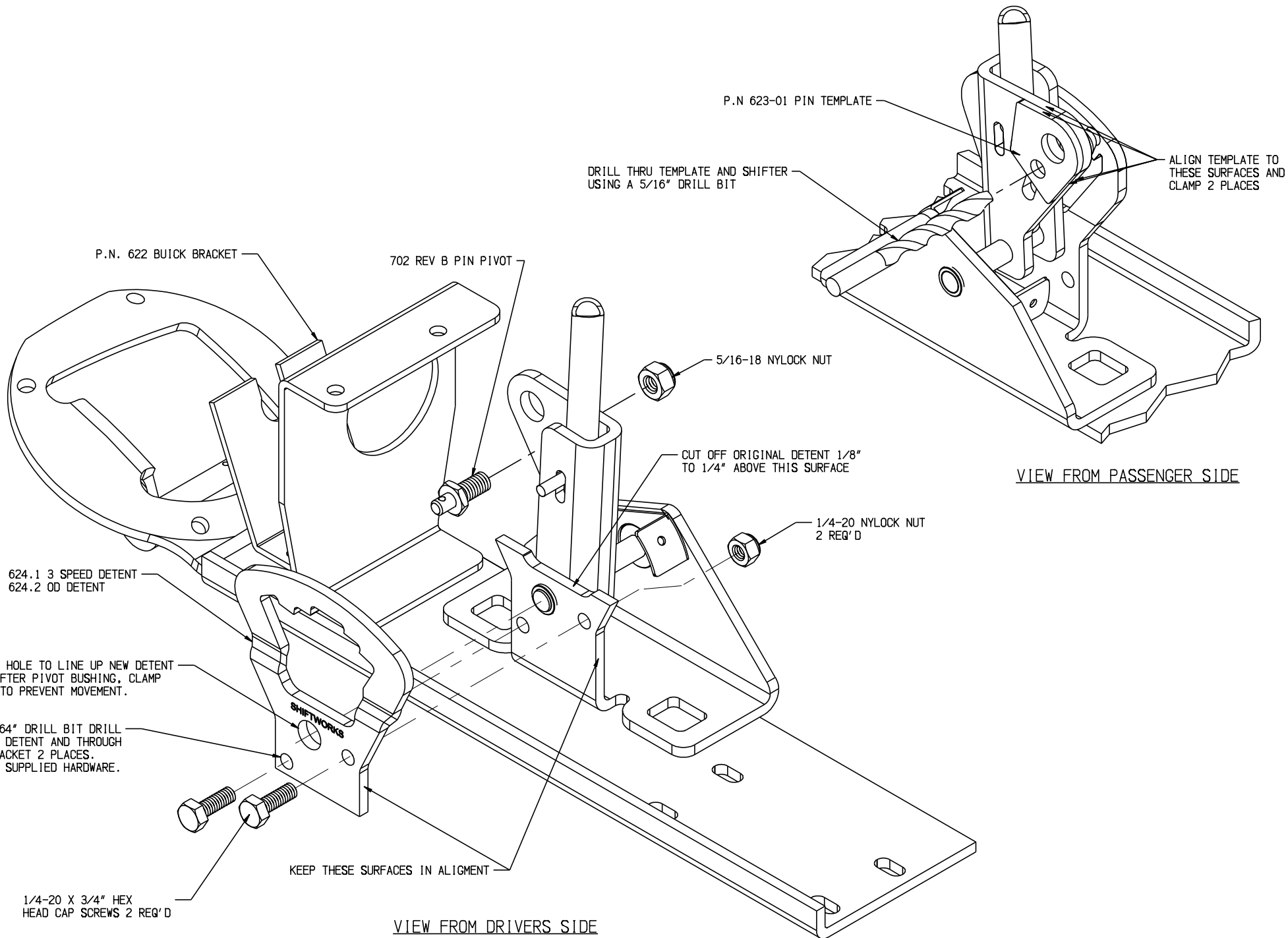
1964-65 BUICK SHIFTER CONVERSION FROM ROD TO CABLE TYPE revised 02-16-18
