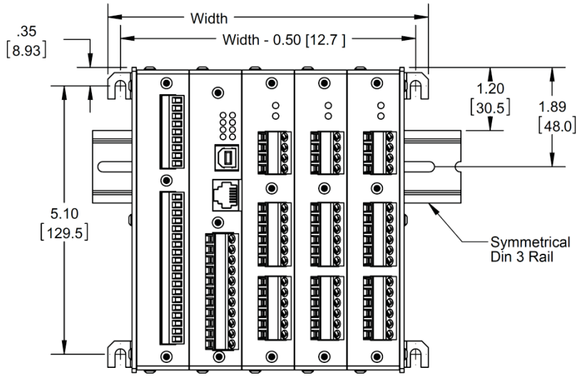
Chassis Front View
