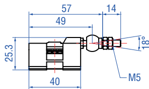
Magnet slider V Part no. 252 184
