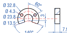
U-magnet OD33 Part no. 251 416-2
