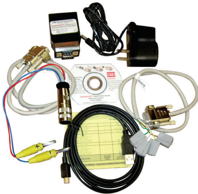
Figure 4. G-Series PC Programming Kit, part no. 253311-1 (Analog) or 253312-1 (Digital-pulse) outputs
