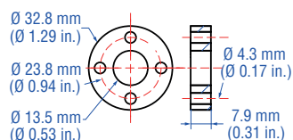
Standard ring magnet Part no. 201 542-2
