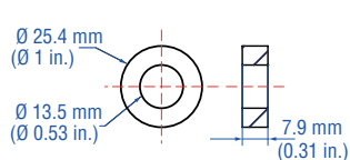
Ring magnet OD25.4 Part no. 400 533
