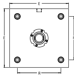
STYLE M—Tie Rods Extended Head End (NFPA Mounting Style MX3)
