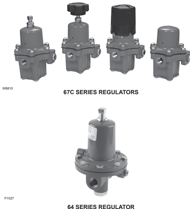
Figure 1. 64 and 67C Series Regulators
