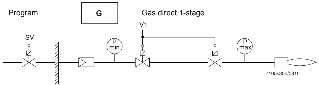
Figure 2: Fuel train gas direct ignition (G), 1-stage
