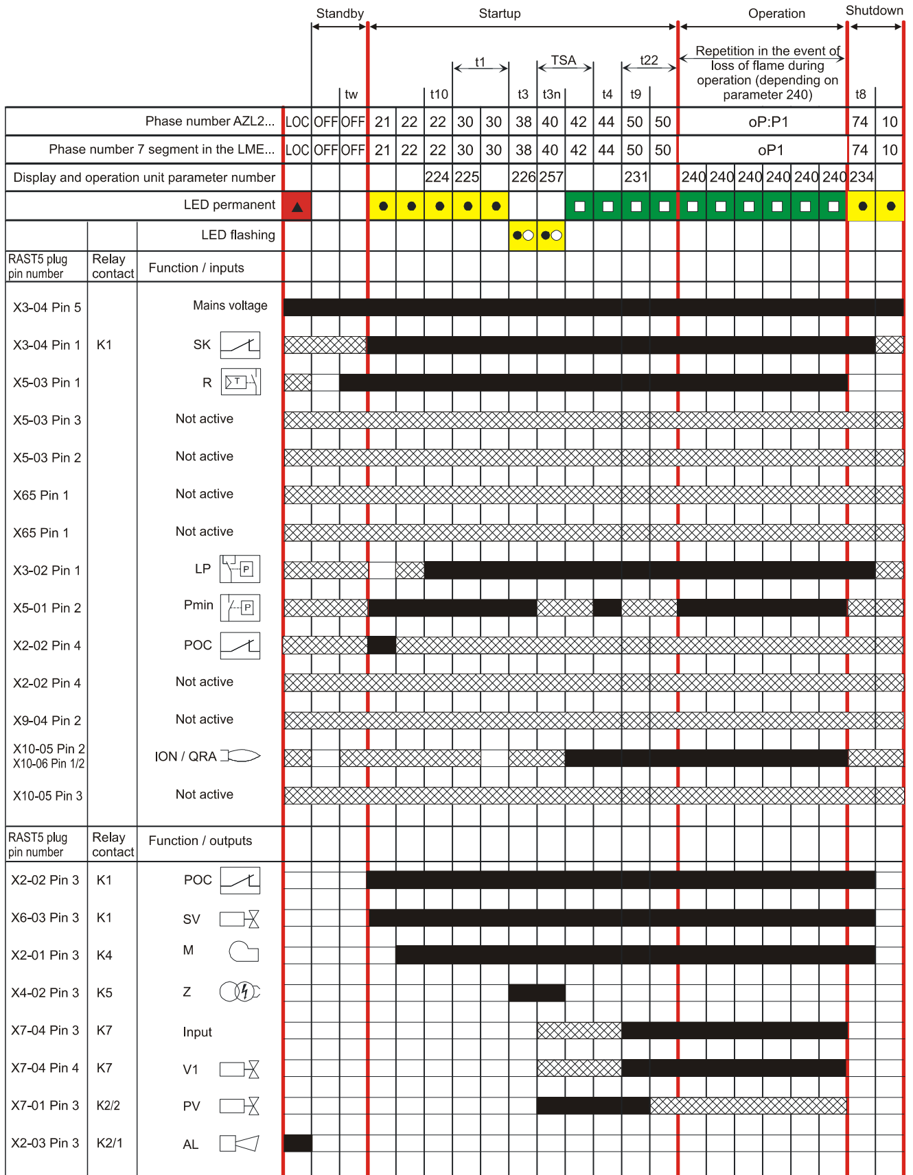
Figure 1: Program sequence
