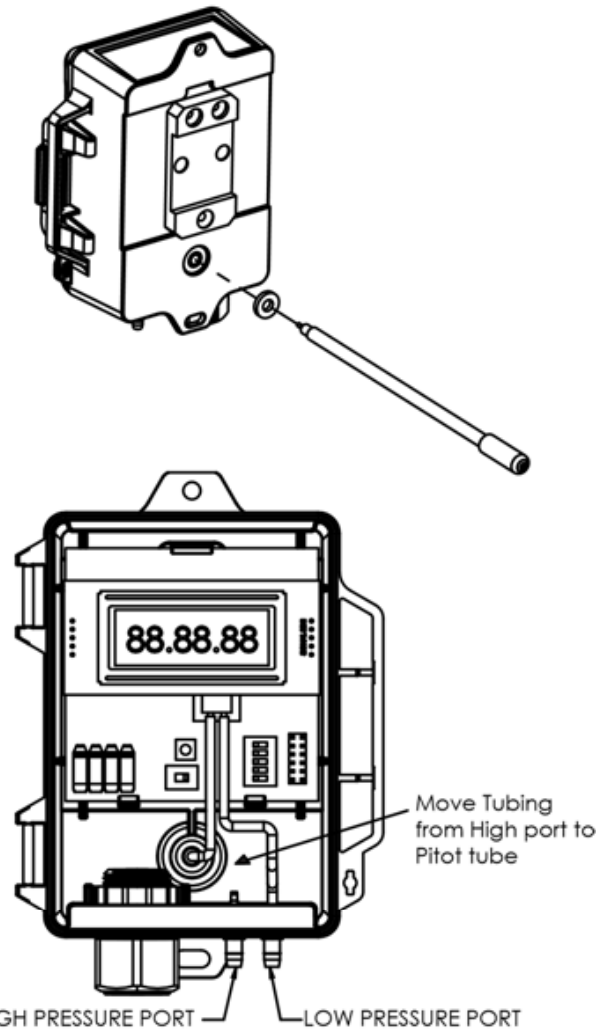
FIGURE 3: PITOT TUBE INSTALLATION
