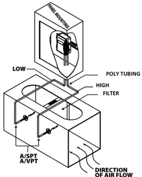
FIGURE 5: MEASURING DIFFERENTIAL PRESSURE ACROSS FILTER
