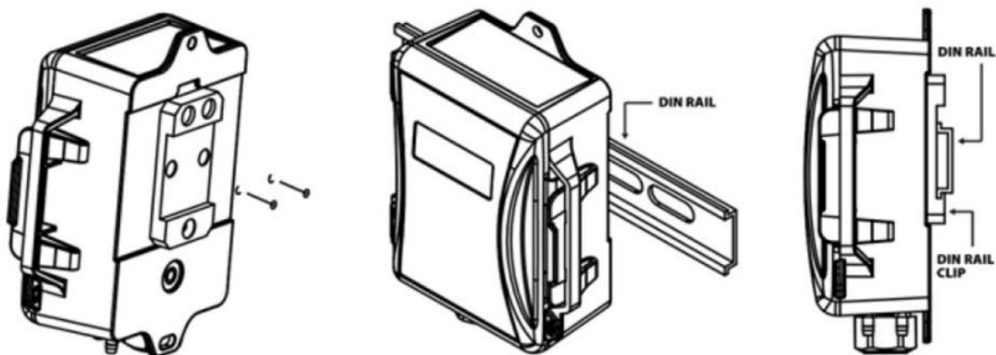
FIGURE 2: DIN RAIL MOUNTING
