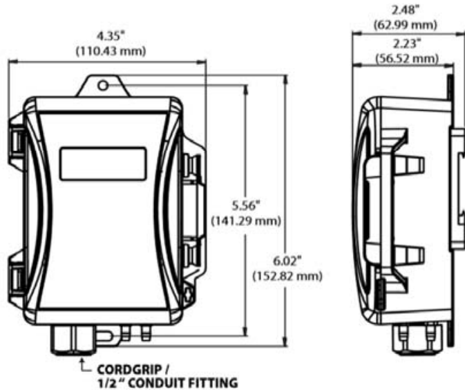
FIGURE 1: DPT DIMENSIONS
