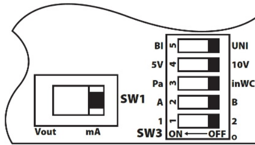
FIGURE 6: SW1 and SW3 OUTPUT SWITCHES
