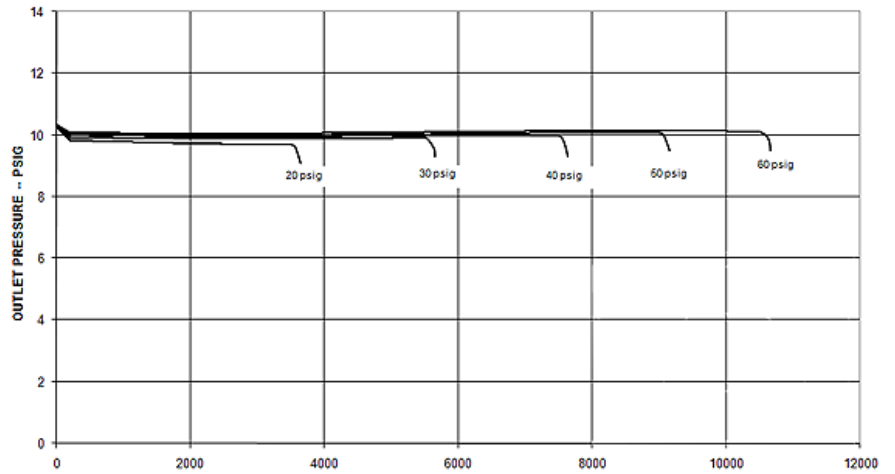
Rate of flow - SCFH 10 PSIG Set Point
