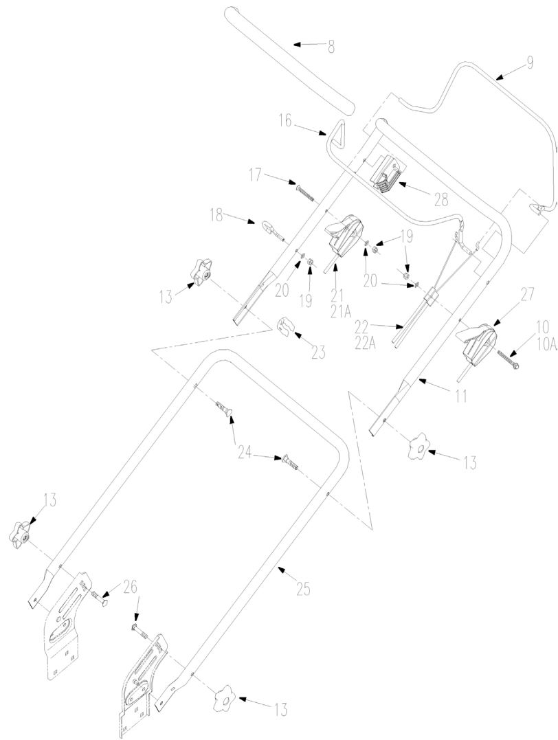
Bluebird Taurus 51TH Rotary Mower
