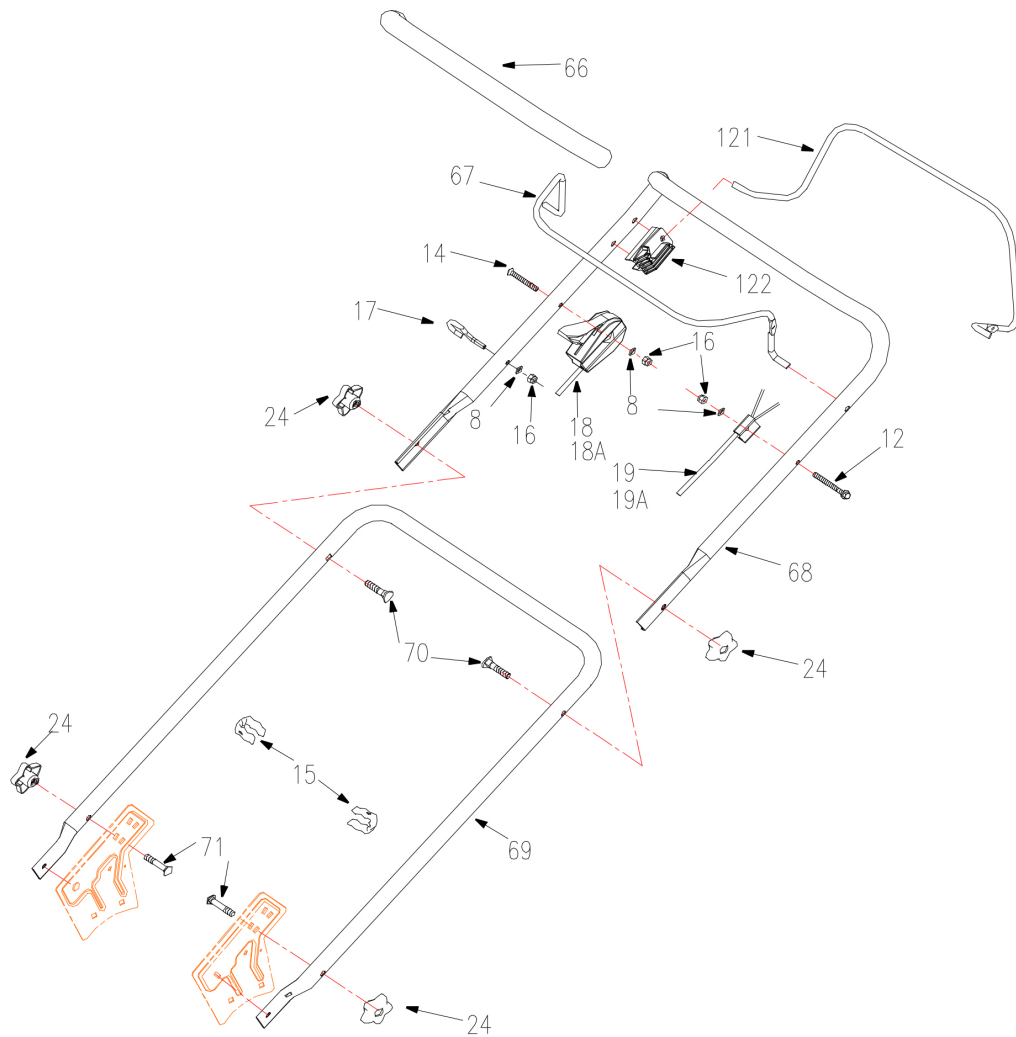
Bluebird Taurus 46TH Rotary Mower
