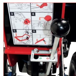
POSITIVE GEAR DRIVE Driven rear wheels even in difficult conditions.
