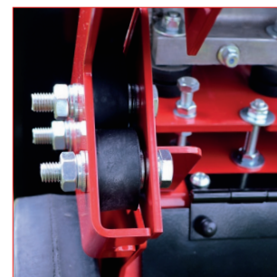
OPTIONAL AV MOUNTS Optional rubber mounted handlebars for further reduced vibration.
