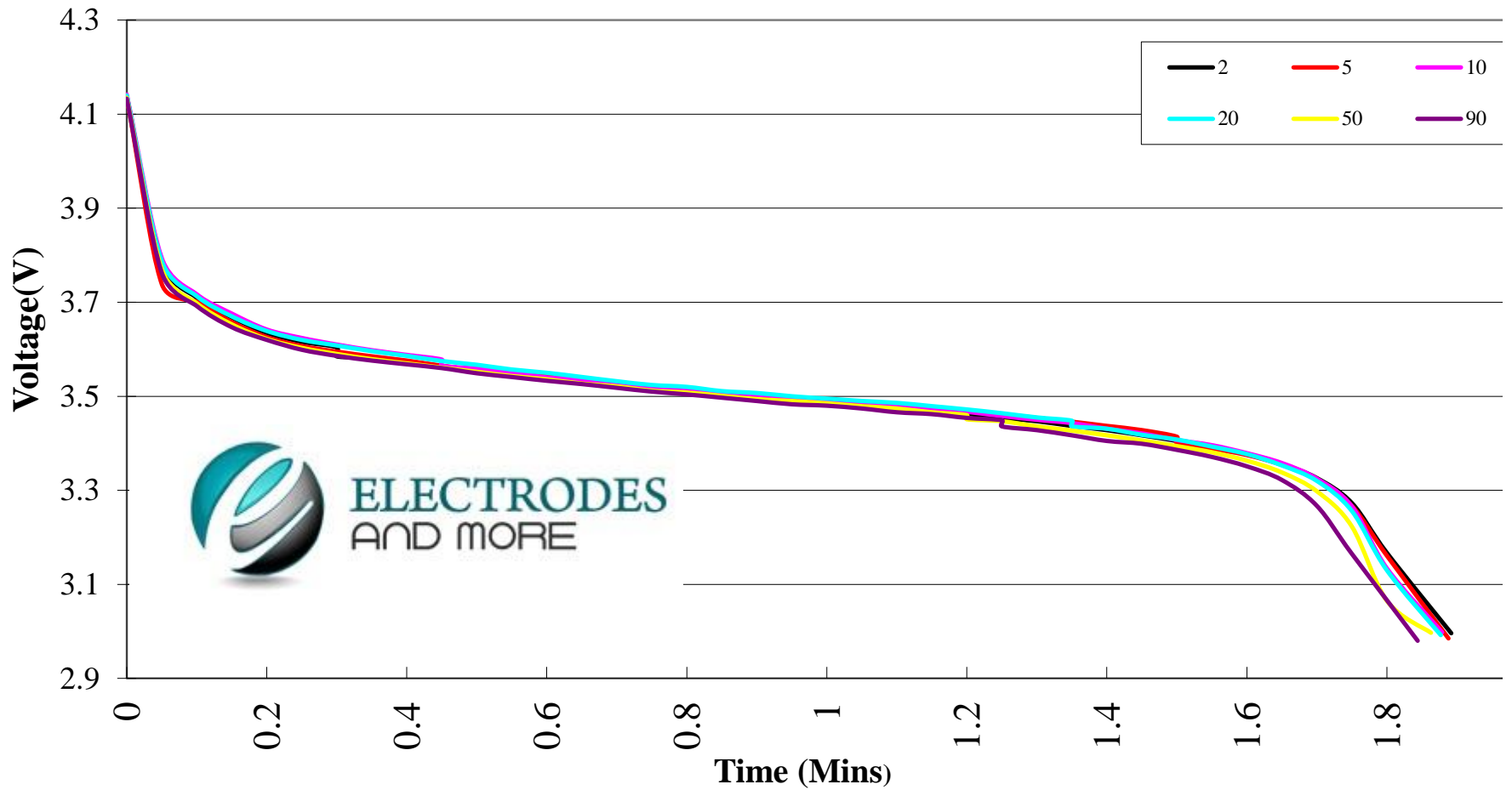
Lithium Cobalt Oxide - LCOP - for Power - Discharge curves at different cycle numbers. 30C rate - Voltage vs Time from Electrodesandmore.com - tested with BCP Anode
