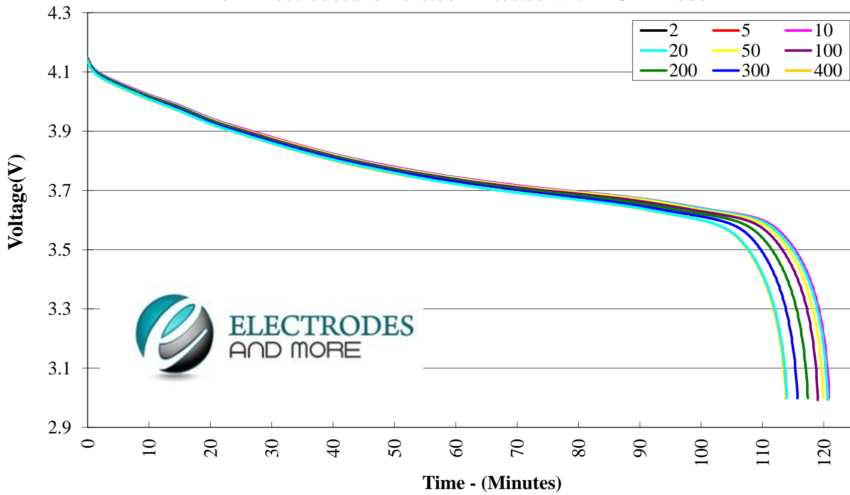
Lithium Cobalt Oxide - LCOE - for Energy - Discharge curves at different cycle numbers. 0.5C rate - Voltage vs Time from Electrodesandmore.com - tested with BCE Anode
