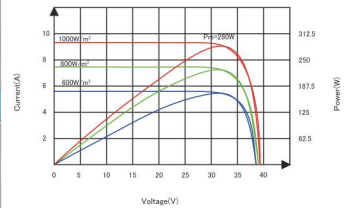
Current-Voltage&Power-Voltage Curve (280W)
