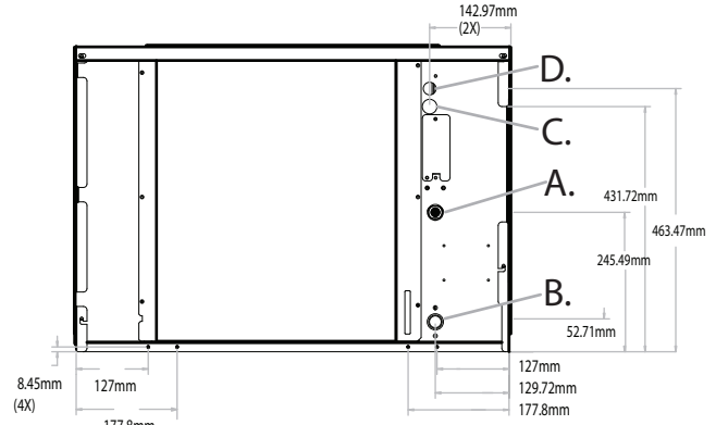
Air Cooled
