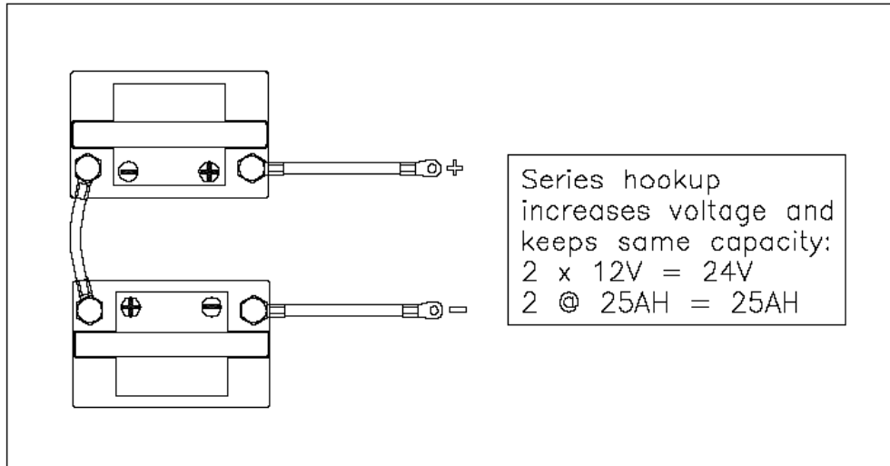
Figure 5-1. Series Connection
