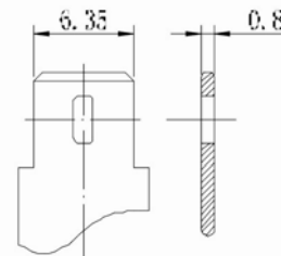
Terminal T2
