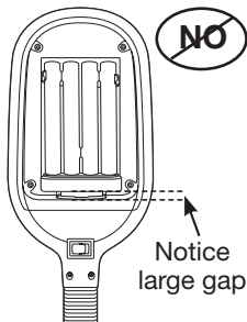
Incorrectly seated bulb
