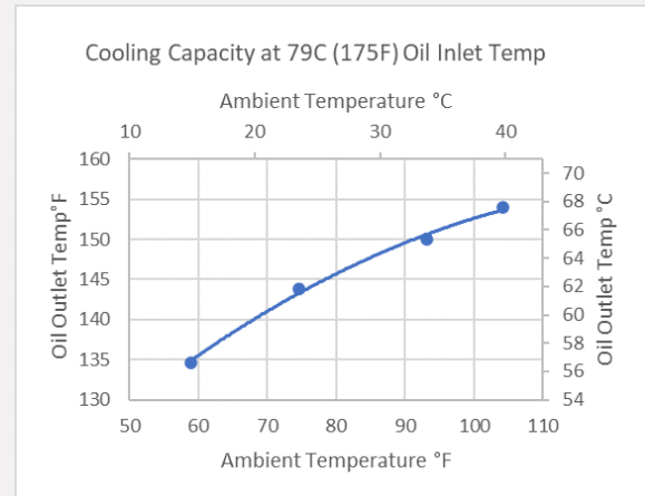
OIL TEMPERATURE
