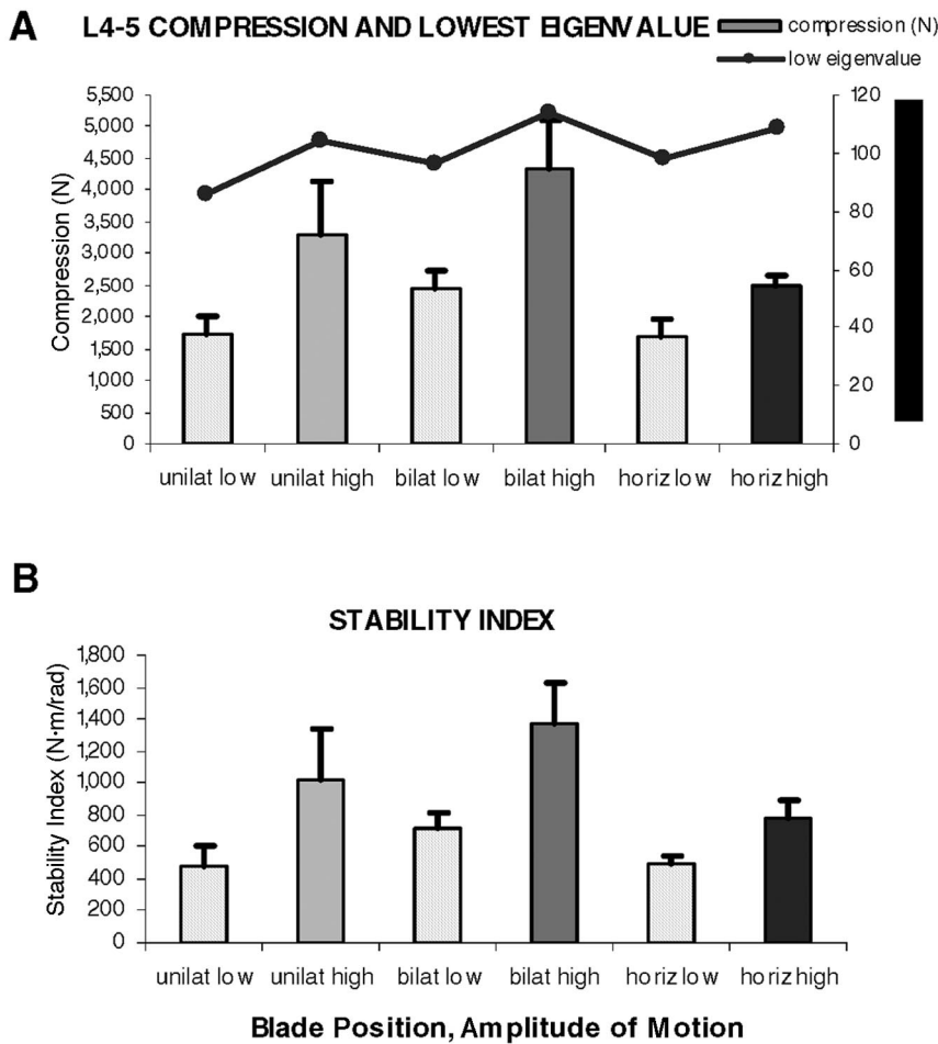
Figure 4. (A) Average ( \pm SD) L4–5 compression and the average lowest eigenvalue for 6 of the Bodyblade trials. (B) Average ( \pm SD) stability index for the same trials. The lowest eigenvalue is indicative of unisegmental lumbar stability, whereas the stability index represents stability of the entire lumbar segment. Unilat=unilateral, bilat=bilateral, horiz=horizontal.
