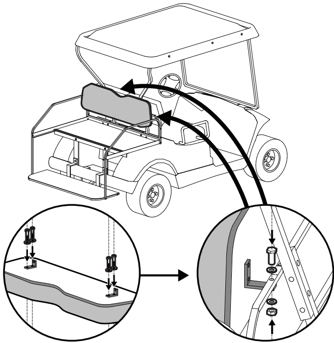
Bolt rear seat supports to back of rear seat back pad using 1/4" x 1" bolts and flat washers.
