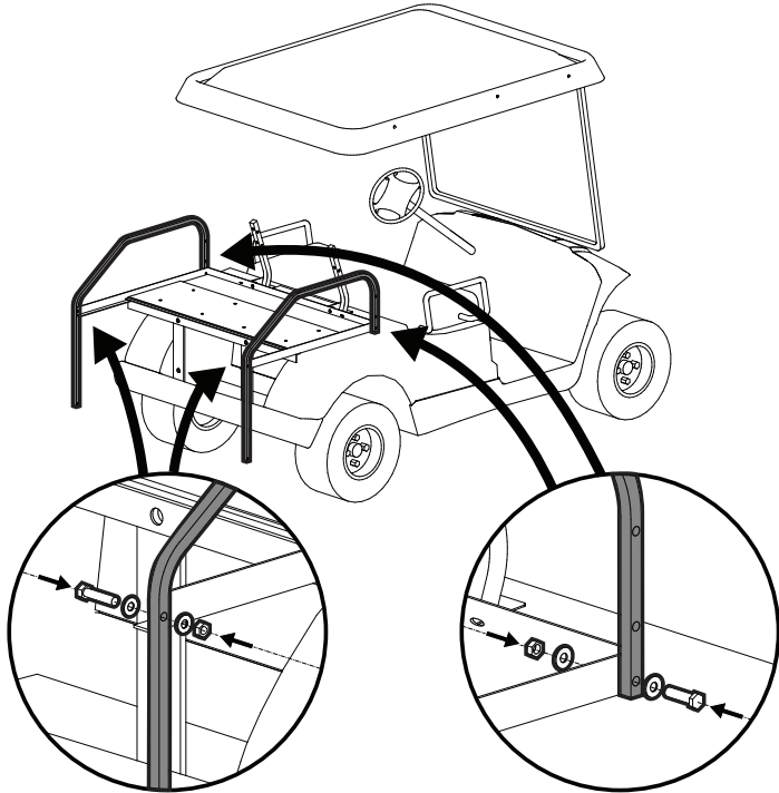
Bolt side rails to rear of flip seat frame with 5/16" x 1 1/2" bolts, flat washers, and acorn nuts.
