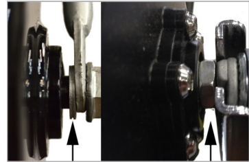
Some motors use a tabbed washer. It faces down and through the dropouts. All motors use an inside washer or lock nut
