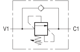
Hydraulic Symbol
