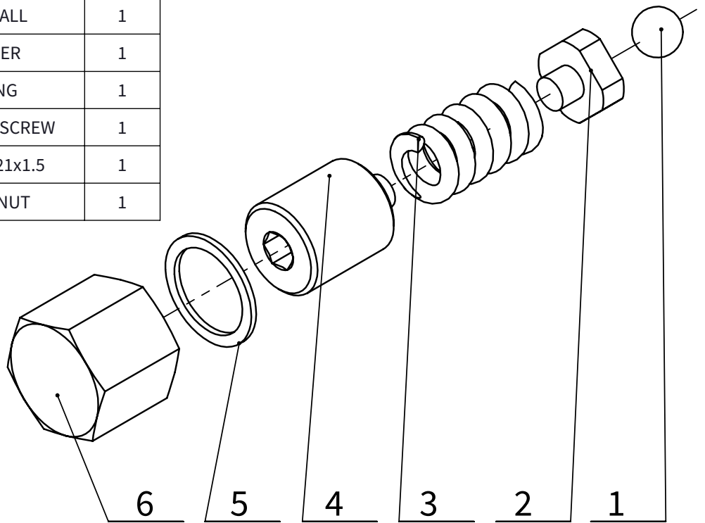
An adjustable ball spring relief valve
