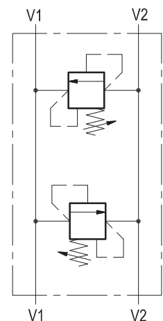
Hydraulic Symbol
