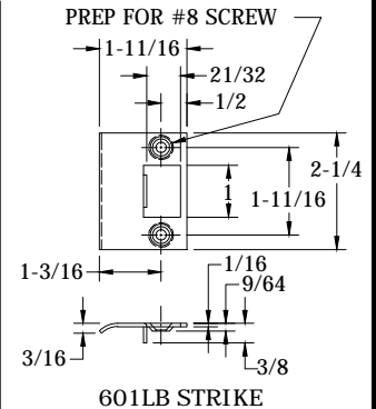
601LB STRIKE
