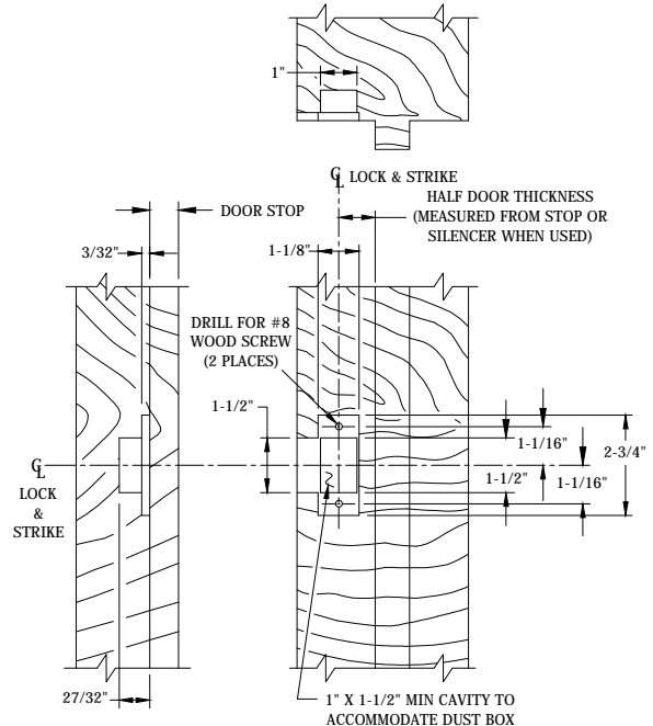
WOOD FRAME (\"T\" STRIKE SHOWN FOR EXAMPLE)
