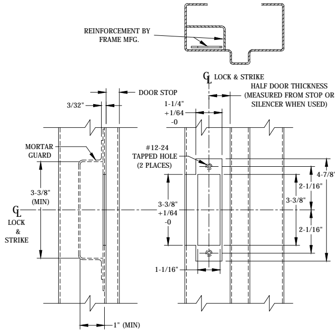
METAL FRAME (ASA STRIKE SHOWN FOR EXAMPLE)
