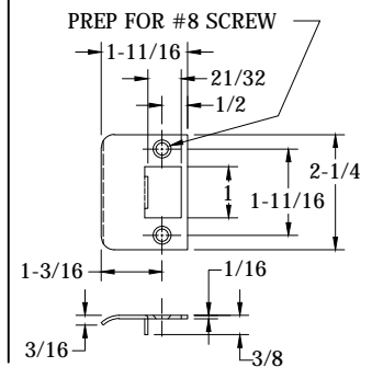
"D" STRIKE
