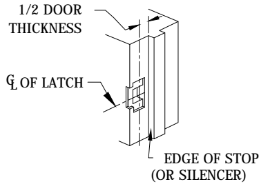
WOOD FRAME (\"T\" STRIKE SHOWN FOR EXAMPLE)
