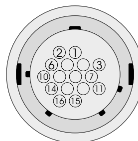
16-way CPC connector - Front view
