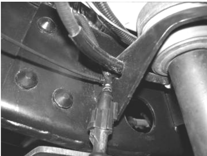
28. Locate FT30402 (08-10) or FT30583BK (11-UP) steering stabilizer drop bracket and install in the factory location
