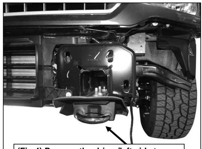
(Fig 4) Remove the driver/left side tow hook and plastic cover, (if equipped)
