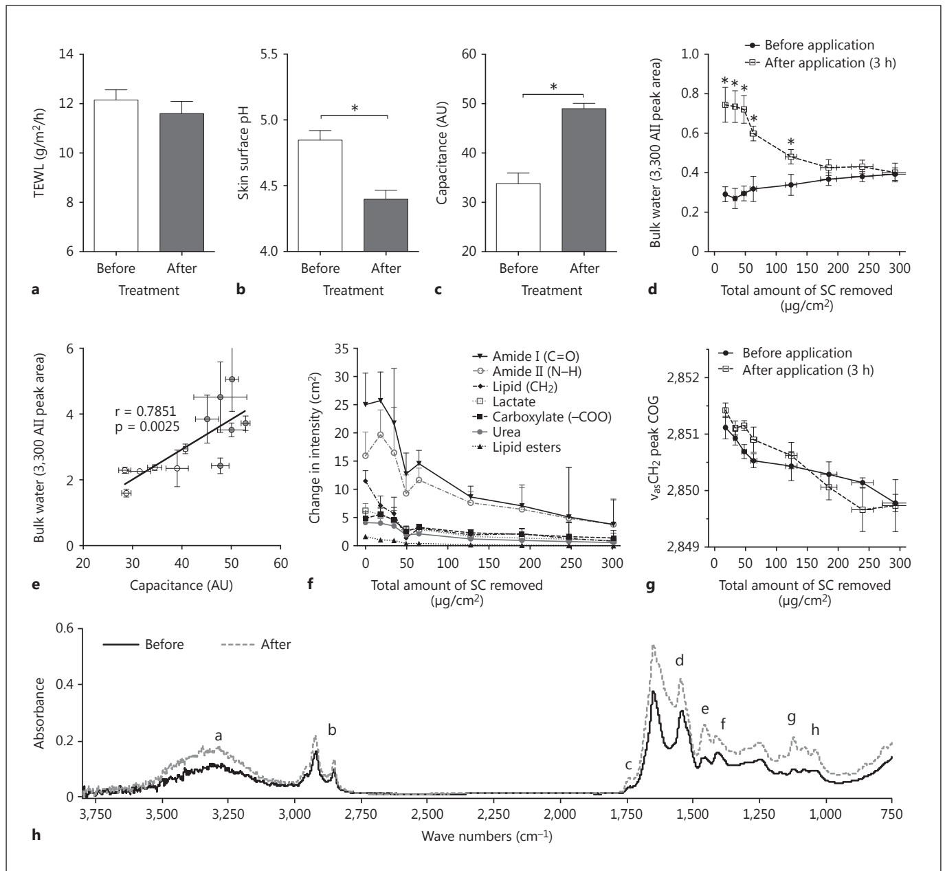
Fig. 3. The effect of a single application of the test emollient on the biophysical properties of the skin: TEWL ( a ), skin surface pH ( b ), and hydration ( c ) before and 3 h following application. d The concentration of water in the SC determined by FTIR spectroscopy before and 3 h following application. Measurements were collected in conjunction with tape-stripping to remove the uppermost layers of corneocytes and achieve greater depths. Two-way ANOVA reported a significant effect of test emollient treatment (and the interaction between treatment and tape strip number) on SC water content. AII = Amide II. * p < 0.05 . e Correlation between water concentration and capacitance (Pearson coefficient shown). Open circles correspond to measurements taken before treatment and filled circles to measurements taken after treatment. AII = Amide II. f The change in concentration of key functional groups
