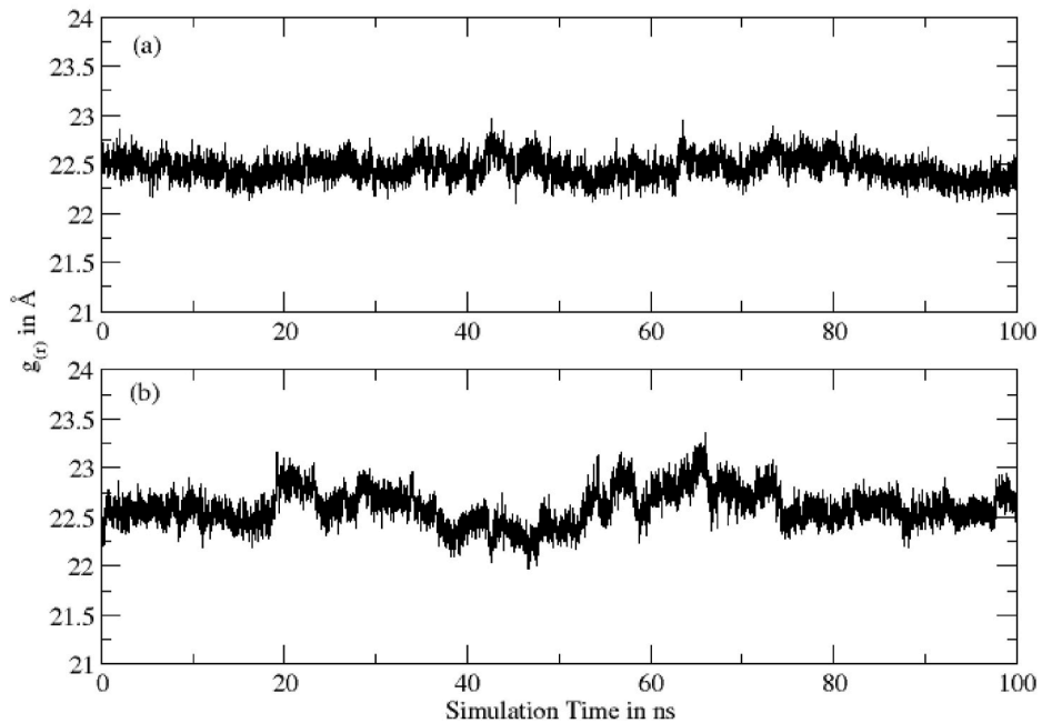
Fig. 8. ROG calculated (a) Hinokiflavone = 22.46 \pm 0.12 Å and (b) Myricetin = 22.60 \pm 0.18 Å.
