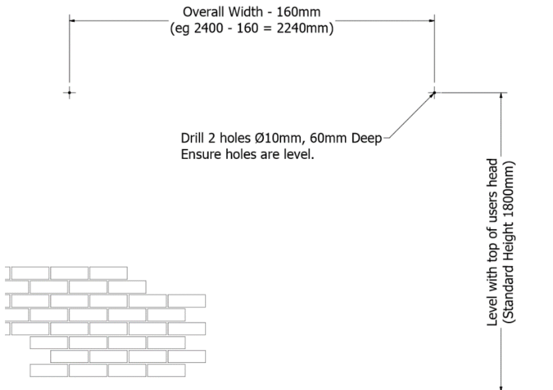
Figure 1 – Layout.
