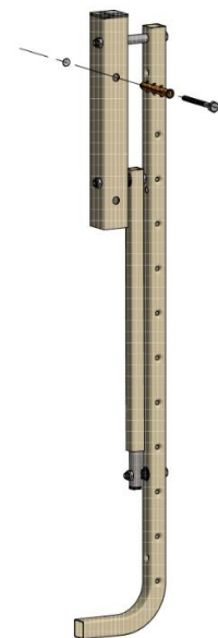
Figure 2 – Mount Arm Assembly
