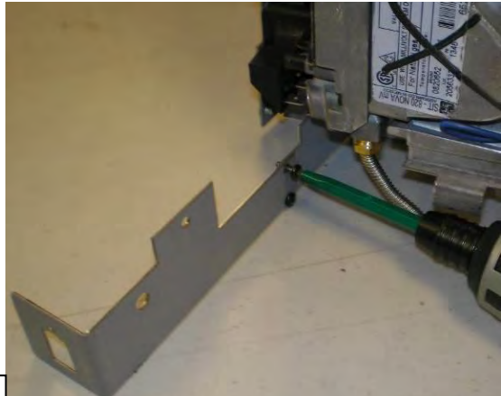
2 Attach On/ Off Switch Extension Bracket using [2] #6 Combo Screws as shown.
