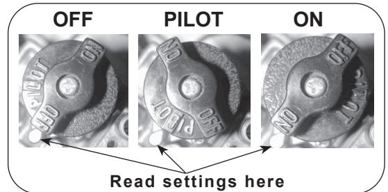
Fig. 19-2 12 valve operating positions
