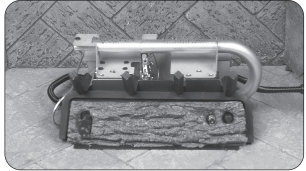
Fig. 20-2 Install decor cover (12 valve)
