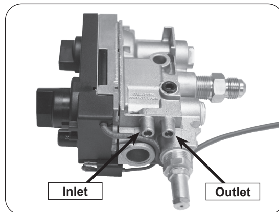
Fig. 23-3 15 valve: check pressure
