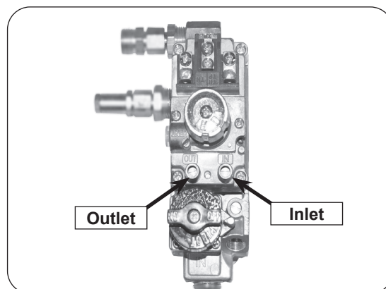
Fig. 23-2 12 valve: check pressure
