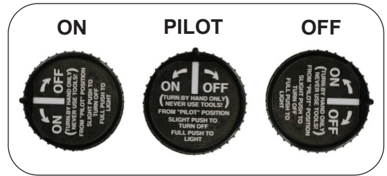
Fig. 19-1 Manual valve operating positions
