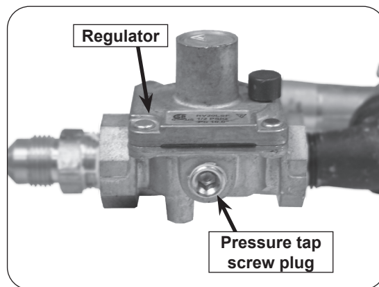
Fig. 23-1 Manual valve: check pressure
