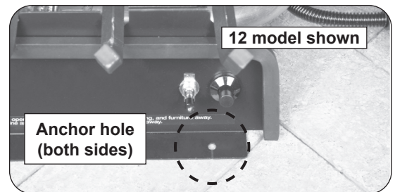
Fig. 19-4 Secure burner to floor (if required)
