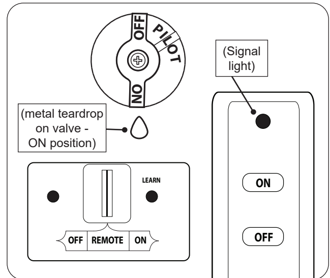
Fig. 29-1 Remote lighting
