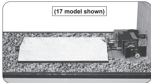
Fig. 19-1 Place sand/vermiculite
