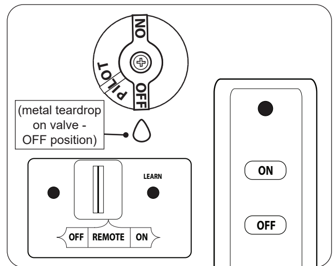
Fig. 29-2 Remote shut down
