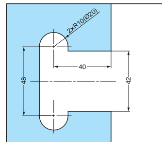
Bore Dimensions
