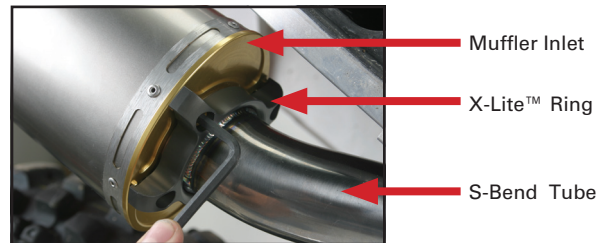
V.A.L.E.™ Assembly Detail
