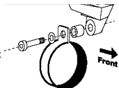
Canister Clamp Detail
