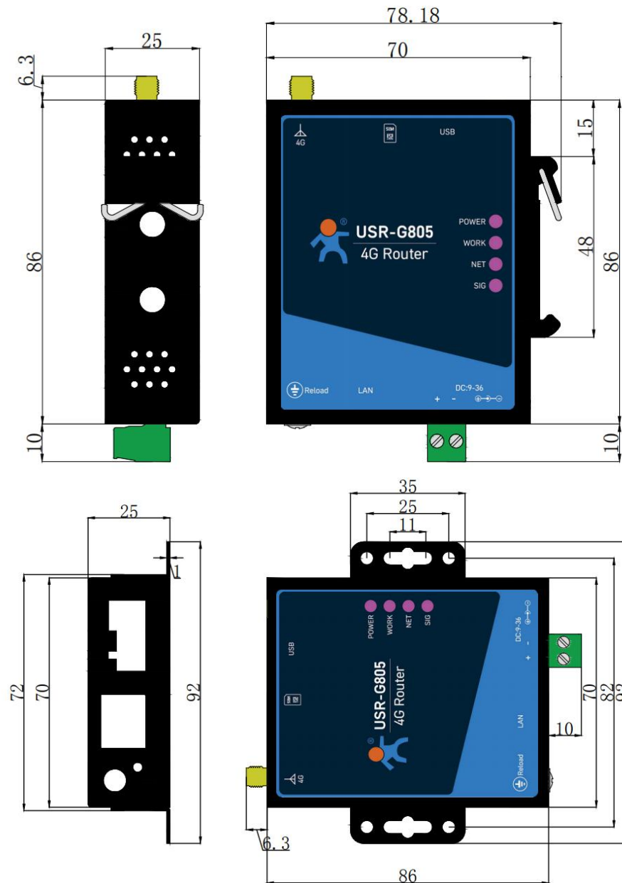
USR-G805 Dimensions
