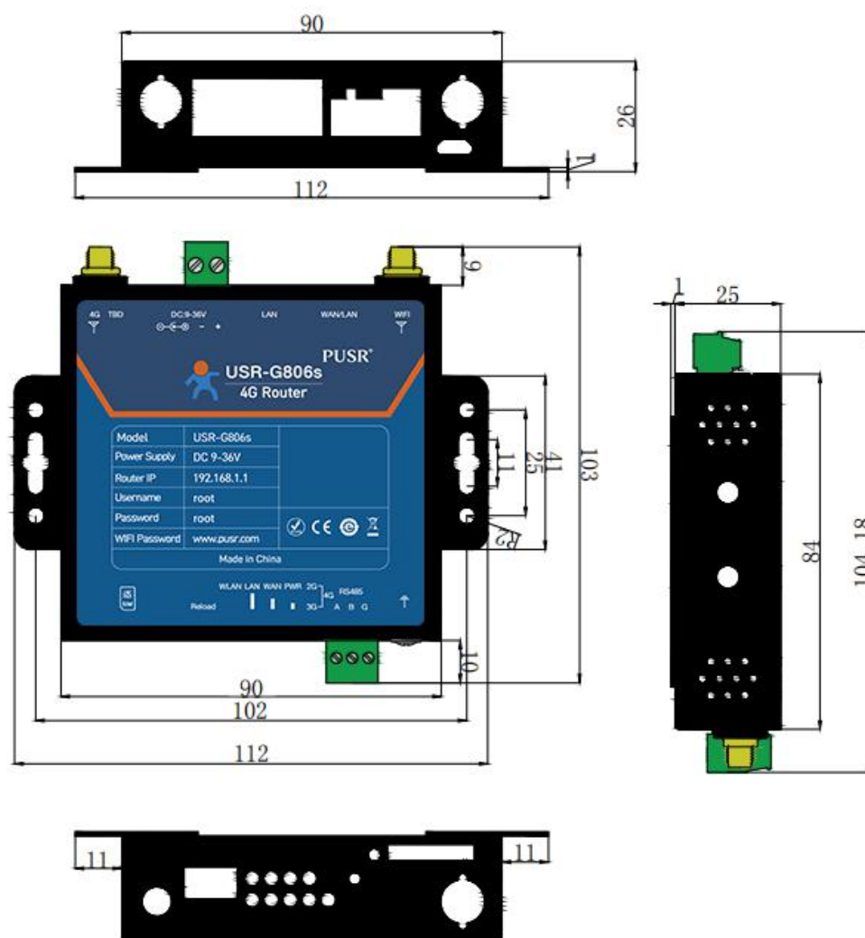
USR-G806s Dimensions
