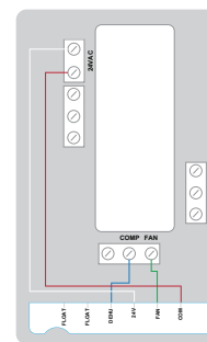
QUEST DEH 3000R CONTROL WIRING DIAGRAM
