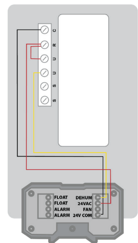
HONEYWELL HUMIDIPRO WIRING DIAGRAM
