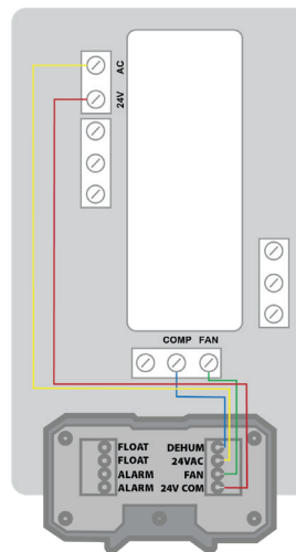
QUEST DEH 3000R CONTROL WIRING DIAGRAM
