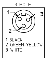
FACE VIEW-FEMALE INSERT
