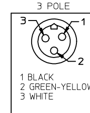
FACE VIEW-MALE INSERT
