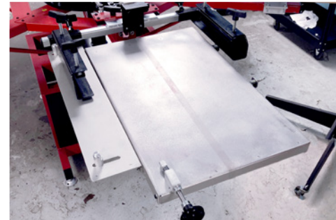
On-Press, 3-Point Screen Receiver
