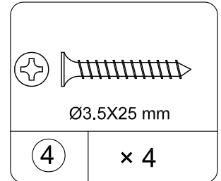
Screw TKX1145
