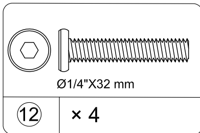
Bolt TKX1009
